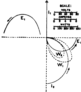
FIG. 8.—Constant Current, Step Down, Arm at 120°
